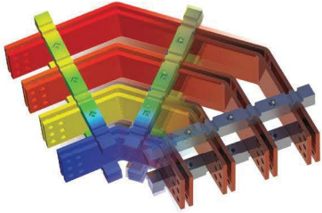
Electric stresses in a bus bar assembly
