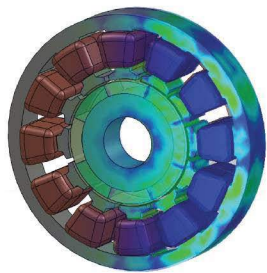
Magnetic flux density distribution in a BLDC motor
